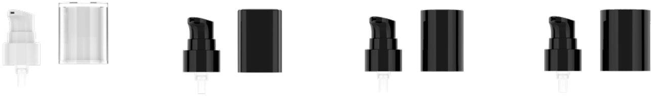
ECLAT Neck 20/400 Dosing 250 mcl Cover ABS + SAN SIDE Neck 20/400 Dosing 250 mcl Cover shiny PP MAKY 30 Neck 20/400 Dosing 250 mcl Cover matt, shiny & metallized PP MAKY 35 Neck 24/410 Dosing 250 mcl Cover matt, shiny & metallized PP
